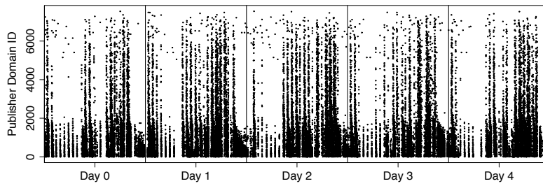
(a) Publisher domains seen from milking via the US over all 5 days of the study.
