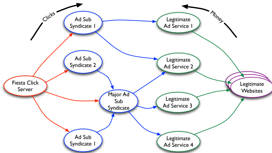
Fig. 4. The expanded Fiesta click redirection chain. This graph represents the possible redirection paths beginning with a click on the Fiesta click-server and ending at a legitimate website. One click will take one path through the graph. Redirections flow from left to right, and money flows from right to left.
