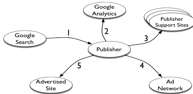
Fig. 7. General progression of a 7cy “job.” Arrows represent HTTP requests and go from the domain of the refer to the domain of the host. Note that the publisher is often a parking page.
