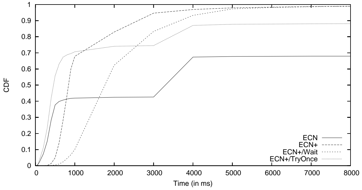
CDF, 10Mb, load 1.5, queue in packets
