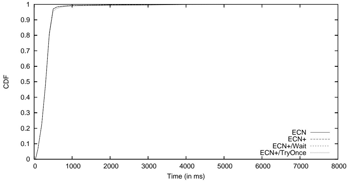
CDF, 100Mb, load 1.1, queue in bytes
