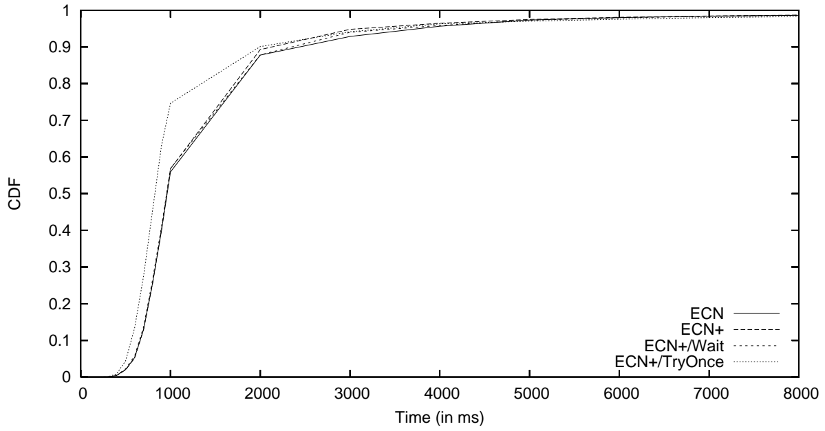
CDF, 10Mb, load 1.5, queue in bytes
