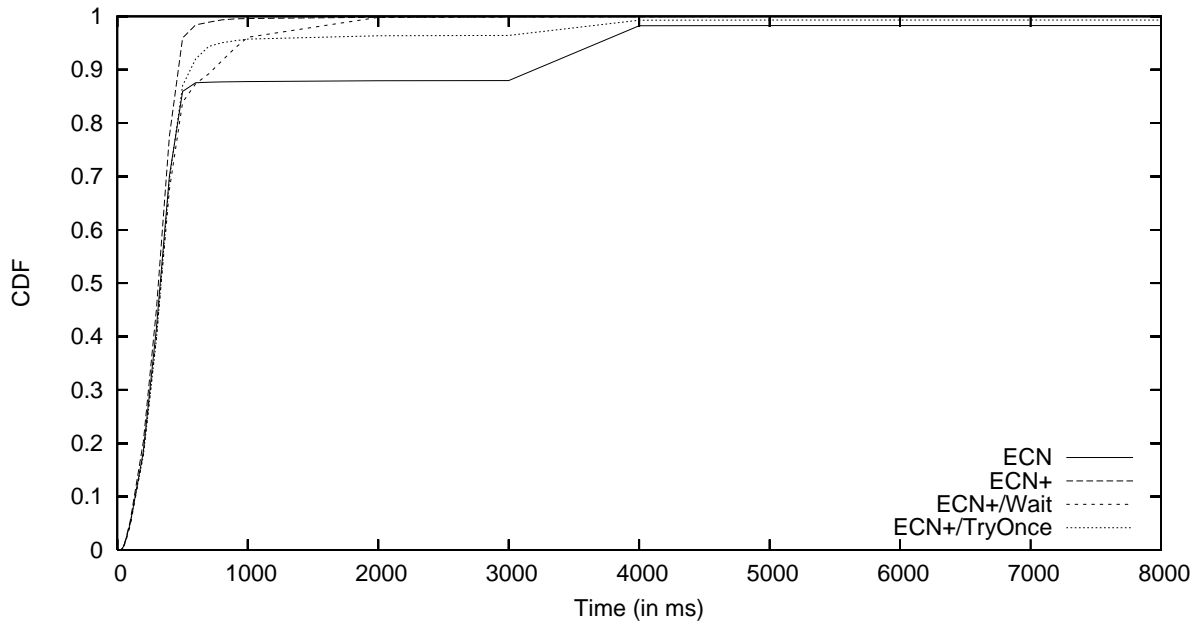
CDF, 10Mb, load 1.1, queue in packets
