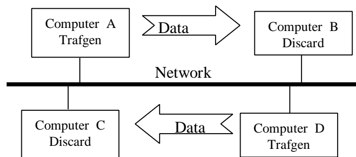
Figure 2: Using trafgen to independently model both sides of a bidirectional traffic flow
