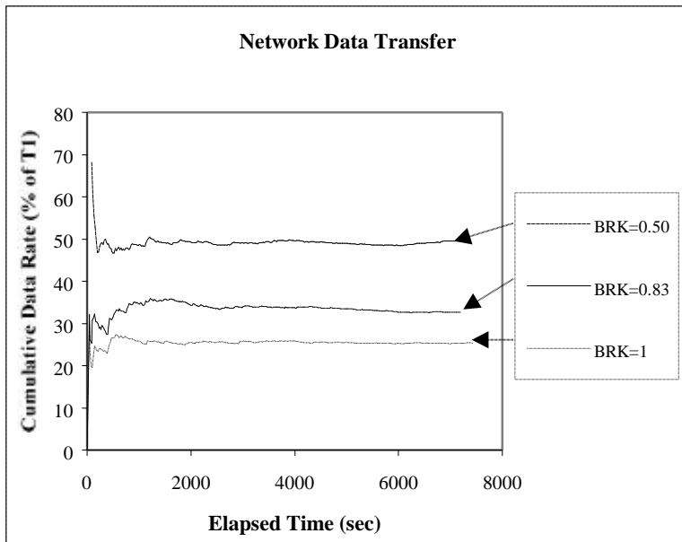
Figure 6: Cumulative data rates observed by the network routers for different BRK settings.
