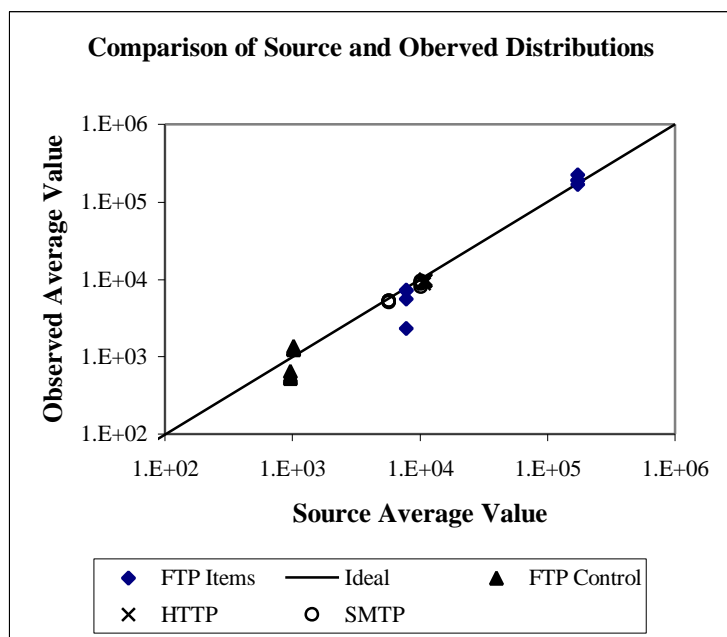
Figure 4: The observed average values for various tclib distributions, plotted as a function of the averages obtained from the source distributions.
