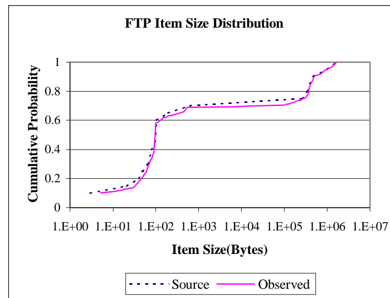
Figure 3: A comparison of source and observed tcplib distributions for FTP item sizes.
