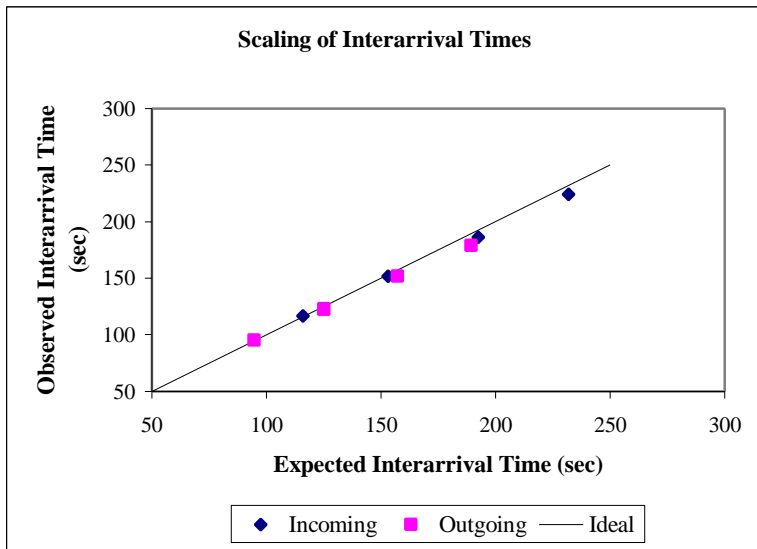
Figure 5: This figure shows the observed average conversation interarrival times against the expected values based on the BRK setting.
