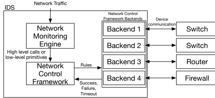
Fig. 1: Basic Architecture.
