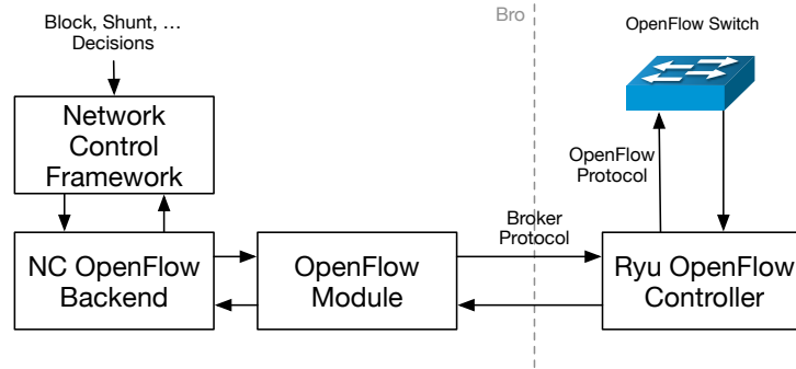
Fig. 2: OpenFlow Architecture.
