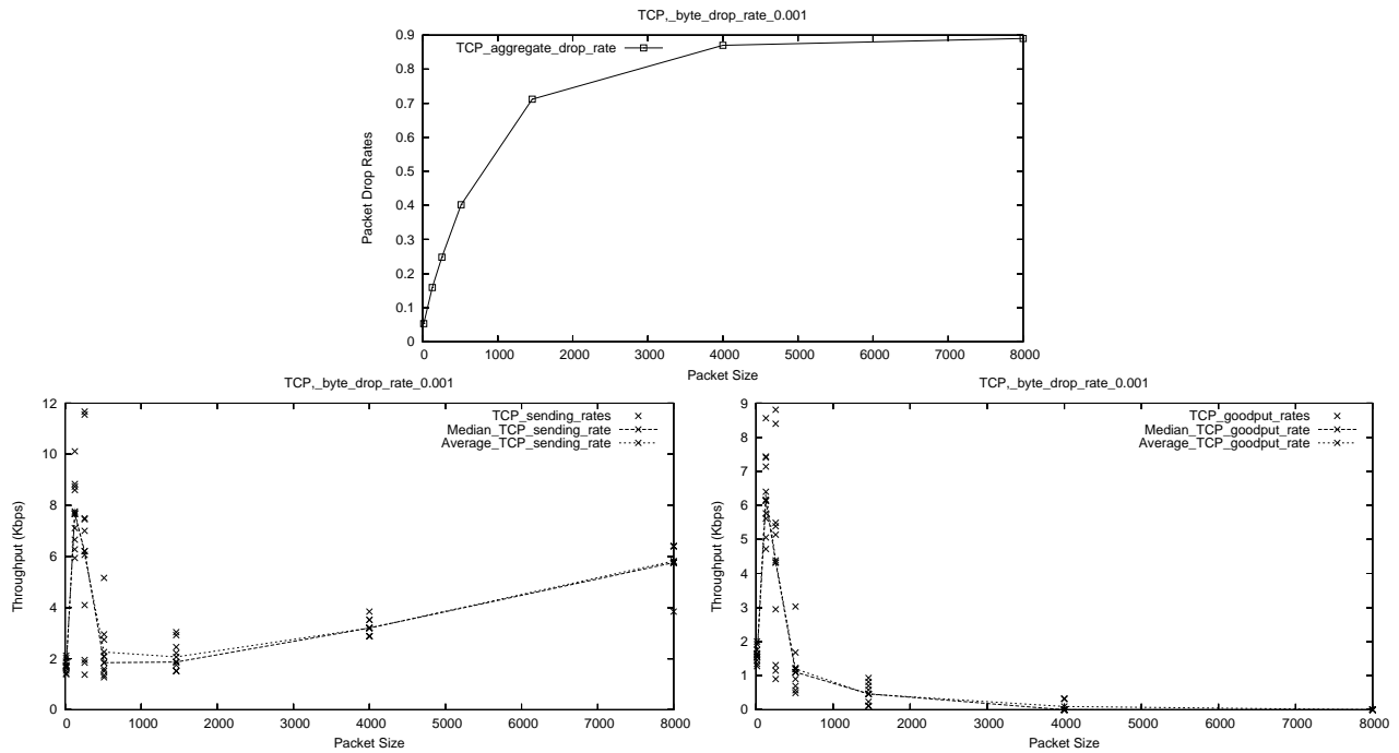
Figure 6: TCP Median Send Rate vs. Packet Size II: Byte Drop Rate 0.001
