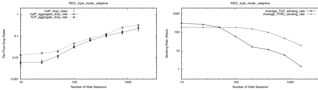
Figure 21: Drop and Send Rates for Adaptive RED Queues in Byte Mode
