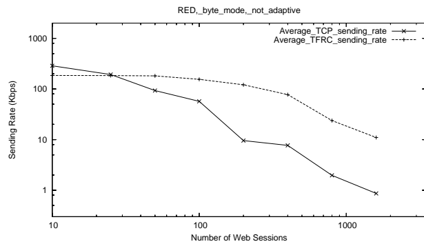
Figure 18: Drop and Send Rates for RED Queues in Byte Mode
