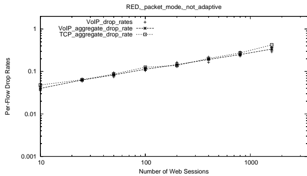
Figure 17: Drop and Send Rates for RED Queues in Packet Mode
