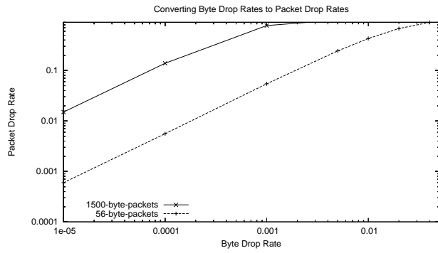
Figure 11: Packet Drop Rate Ratio vs. Byte Drop Rate
