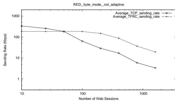
Figure 19: Drop and Send Rates for RED Queues in Byte Mode
