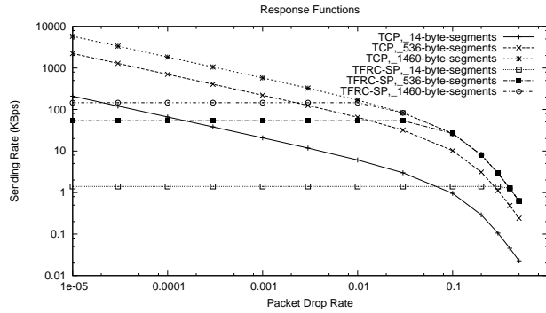
Figure 1: Response Functions for TCP, TFRC, and TFRC-SP. Sending Rate in KBps, as a Function of Packet Drop Rate.
