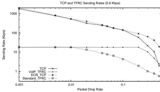
Figure 8: Send Rate vs. Packet Drop Rate II: 14B TFRC Segments (5.6 Kbps Maximum TFRC Data Sending Rate)
