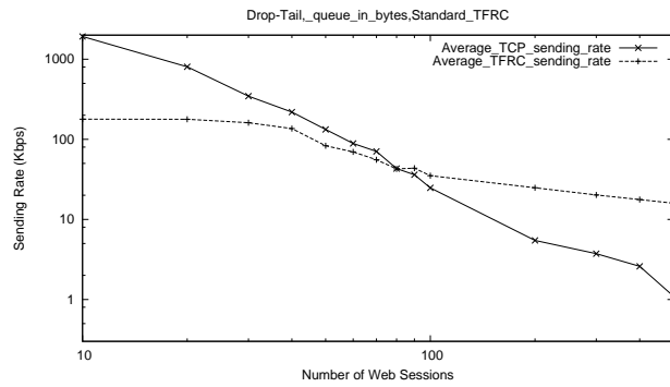
Figure 16: Drop and Send Rates for Drop-Tail Queues in Bytes IV: Standard TFRC, 1460B TCP Segments
