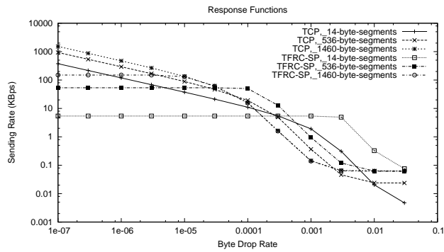
Figure 3: Response Functions for TCP, TFRC, and TFRC-SP. Sending Rate in KBps, as a Function of Byte Drop Rate.
