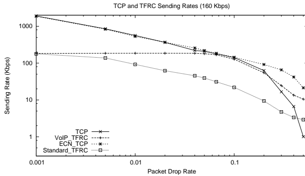
Figure 9: Sending Rate vs. Packet Drop Rate III: 200B TFRC Segments (160 Kbps Maximum TFRC Data Sending Rate)
