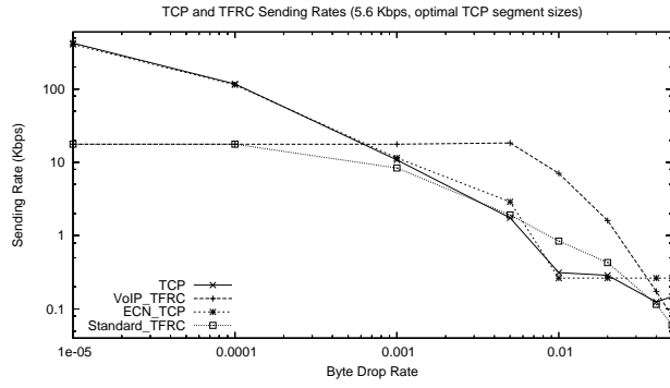
Figure 10: Sending Rate vs. Byte Drop Rate
