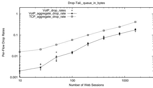
Figure 14: Drop and Send Rates for Drop-Tail Queues in Bytes II: 512B TCP Segments
