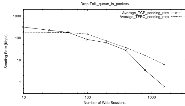
Figure 12: Drop and Send Rates for Drop-Tail Queues in Packets
