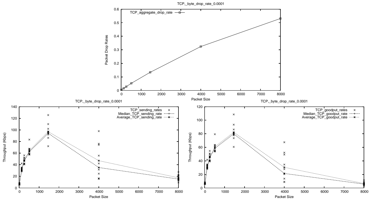
Figure 5: TCP Median Send Rate vs. Packet Size I: Byte Drop Rate 0.0001
