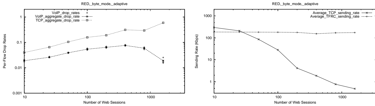
Figure 20: Drop and Send Rates with Adaptive RED Queues in Byte Mode
