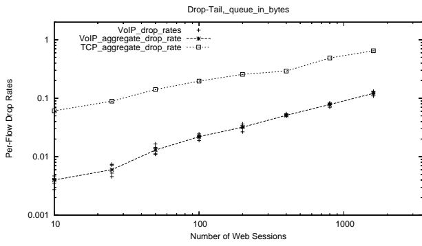
Figure 13: Drop and Send Rates for Drop-Tail Queues in Bytes I: 1460B TCP Segments
