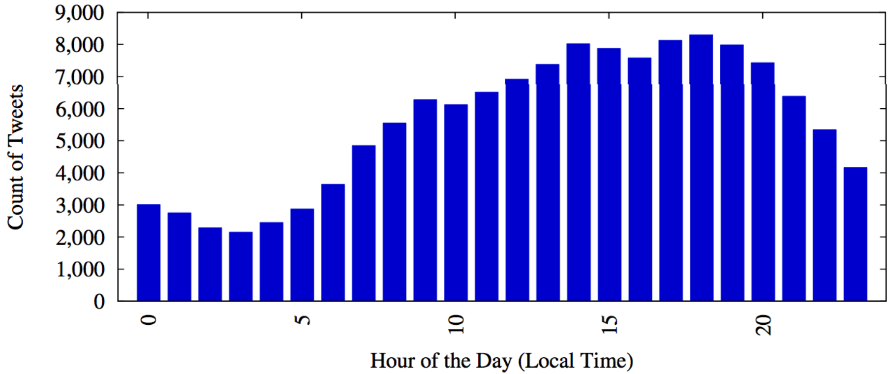
Histogram of Tweets each Hour of the Day
