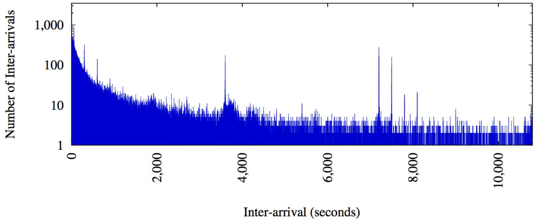
Histogram of Inter-arrival Times
