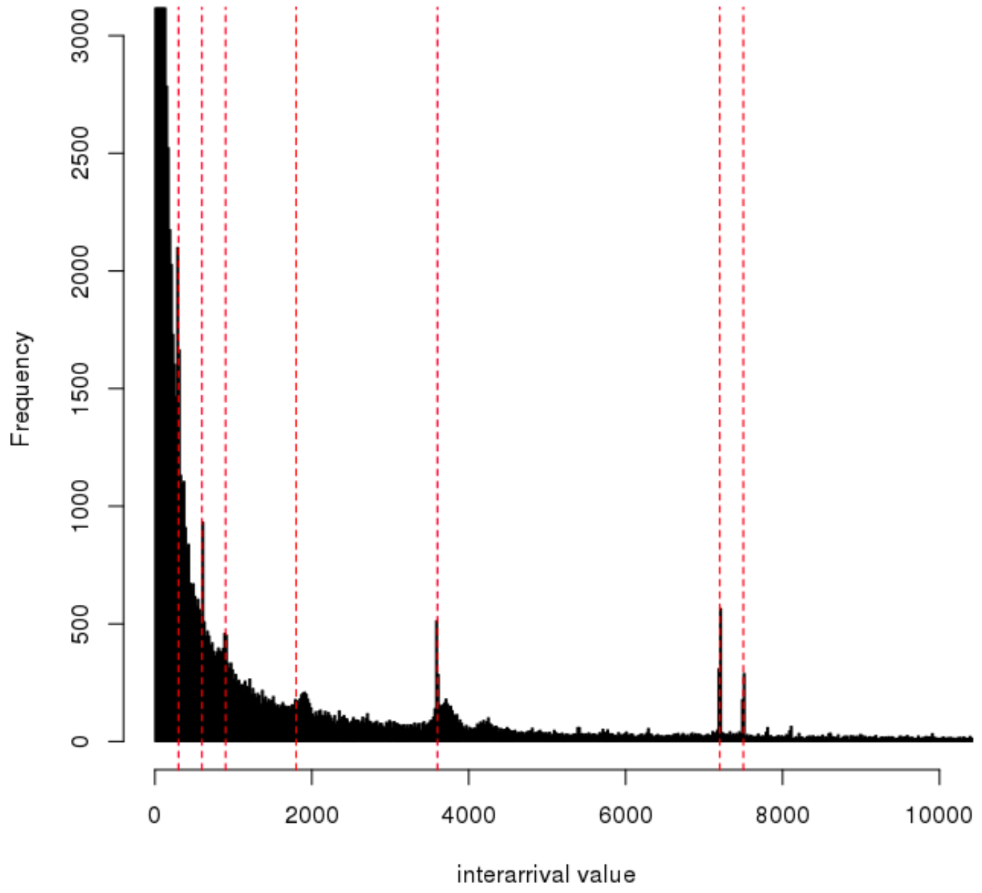
Histogram of tweet interarrivals, all users
