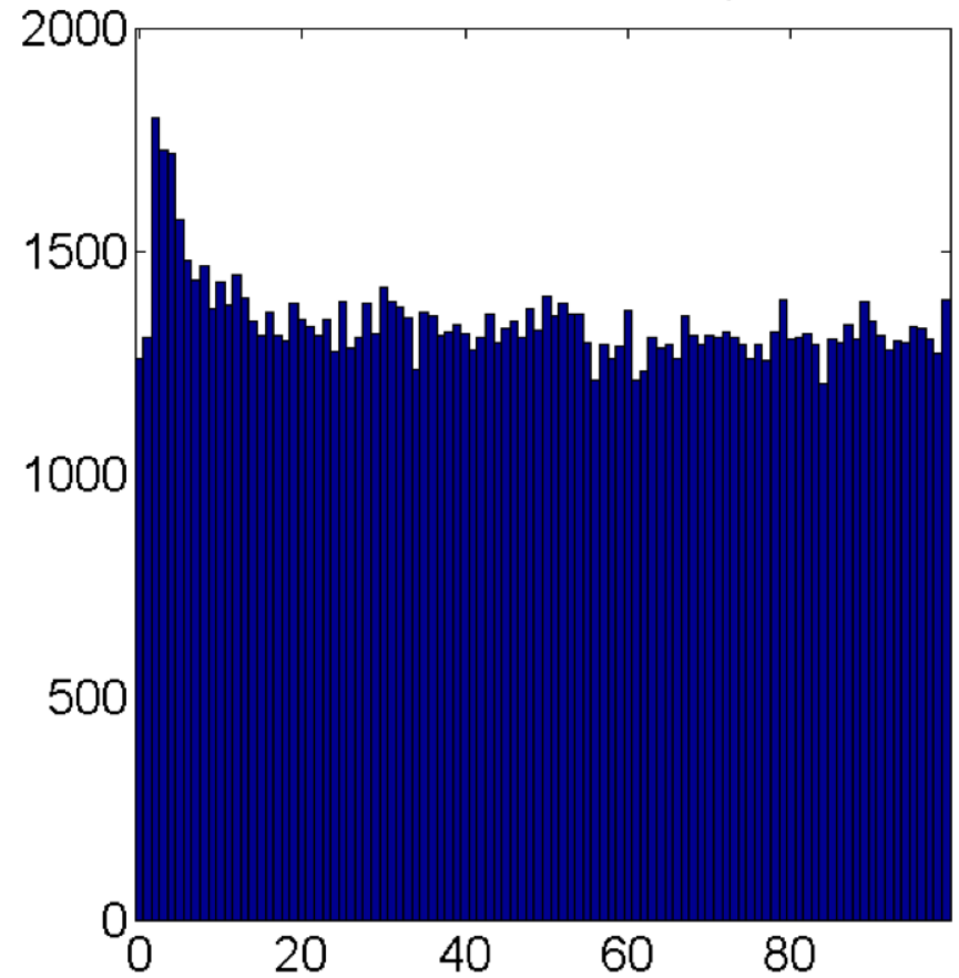
b) Distribution of the last two digits across all timestamps
