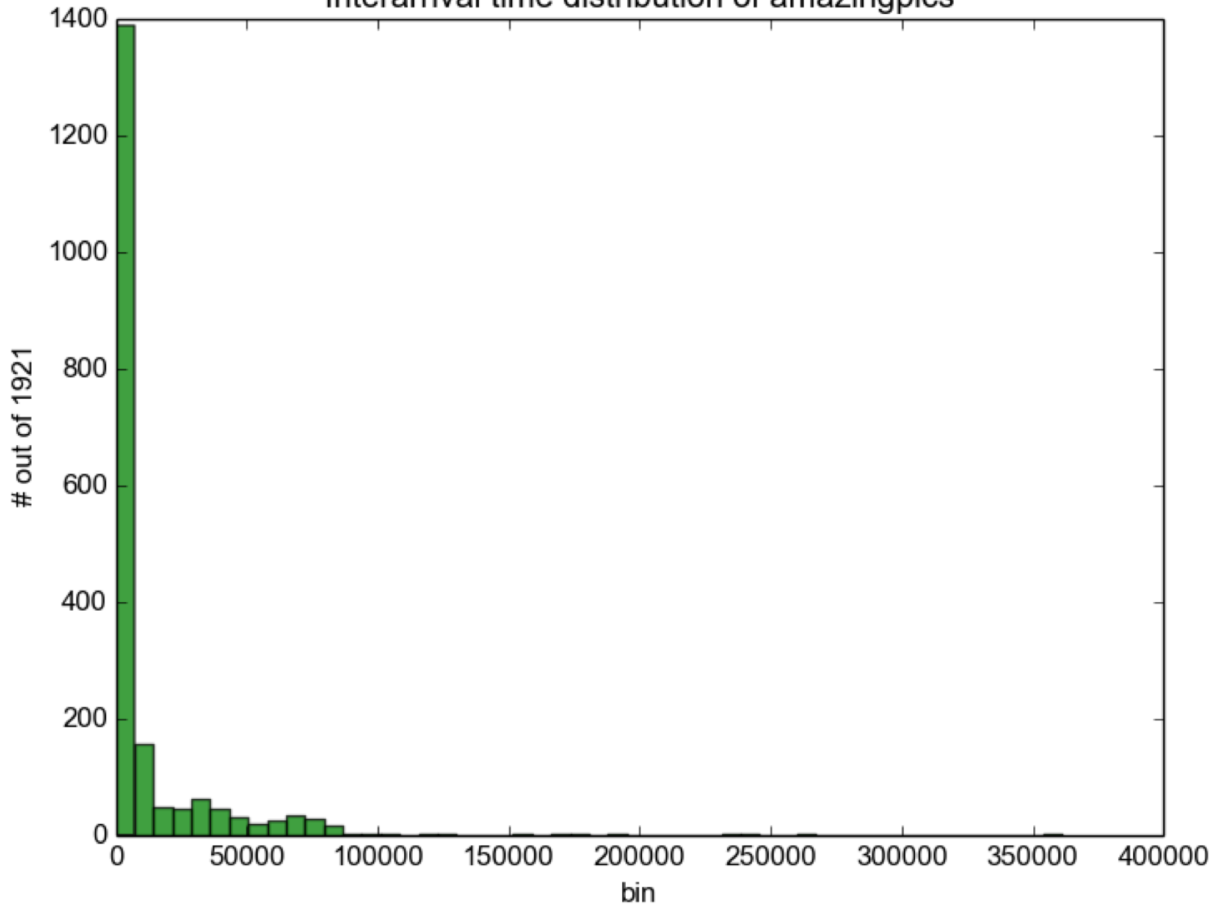
Interarrival time distribution of amazingpics
