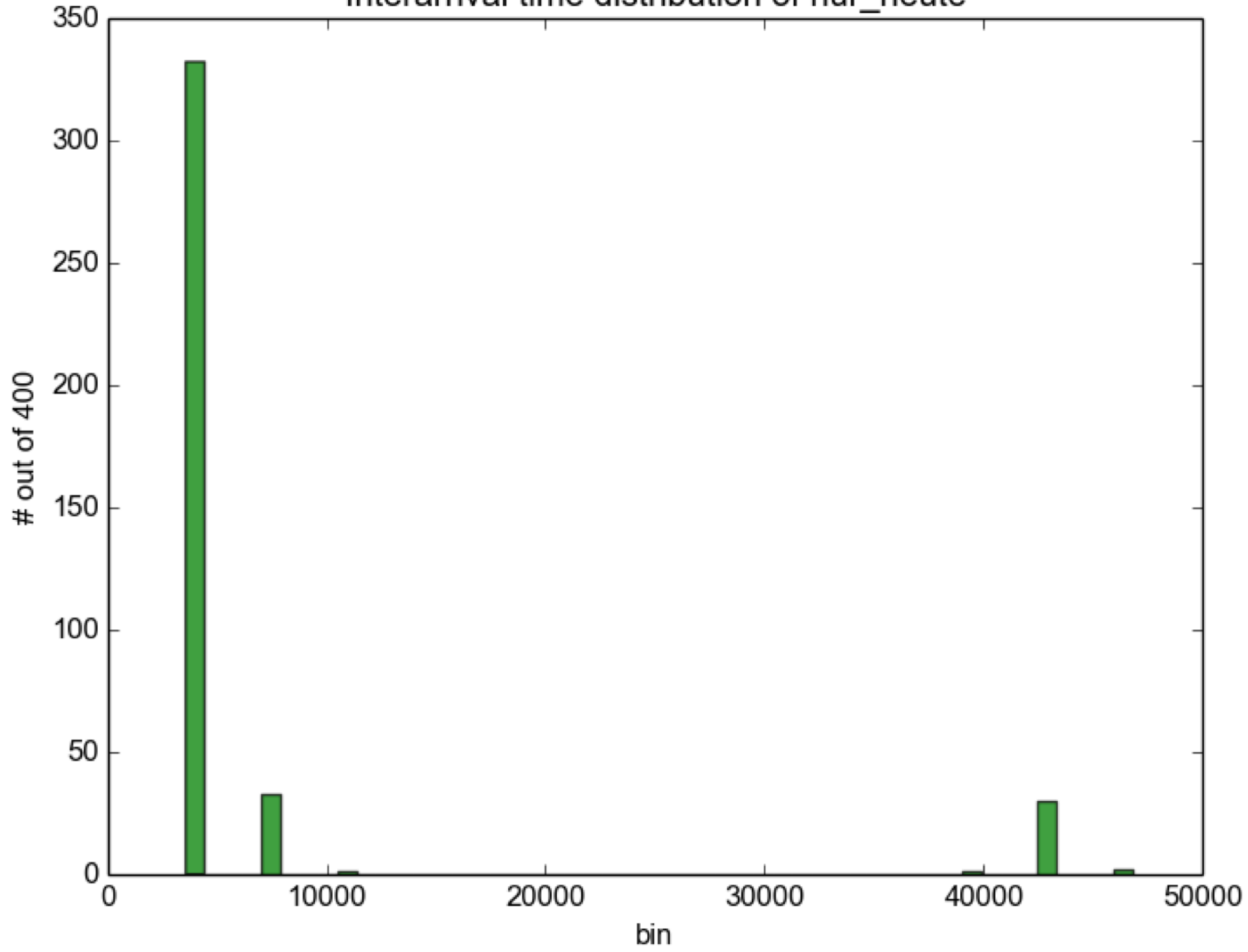
Interarrival time distribution of nur_heute
